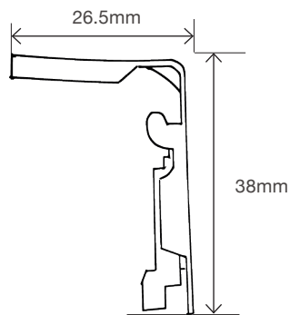
SPRING CLICK UNIVERSAL BRACKET DIMENSIONS
