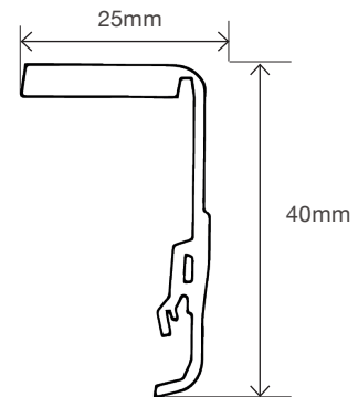
SWIVEL LOCK UNIVERSAL BRACKET DIMENSIONS
